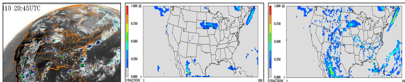
The left panel shows an image of clouds over the United States captured by the weather satellite GOES-13 (20:45 UTC, July 29, 2010). The other two panels show model simulations of cloudiness for the same date and approximate time, first excluding (middle) and then including (right) the effects of thunderstorm clouds on the climate system. Cloud cover in the right panel matches the satellite image much more closely, demonstrating that the new modeling approach better represents the real world—and thus enables greater confidence in regional climate predictions. (Source: Adapted from Alapaty et al., 2012)
