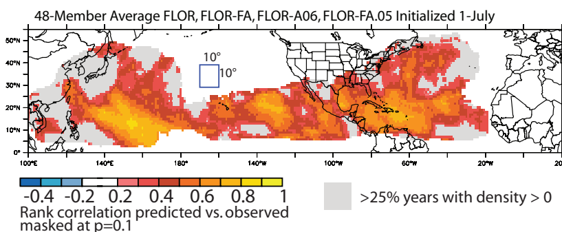
Warm colors on this map show where output from NOAA’s GFDL-FLOR model correlates positively (yellow = strongest correlation) with seasonal observations of tropical cyclone activity, demonstrating the model’s capacity for predicting such phenomena. (Source: Adapted from Vecchi et al., 2014)
